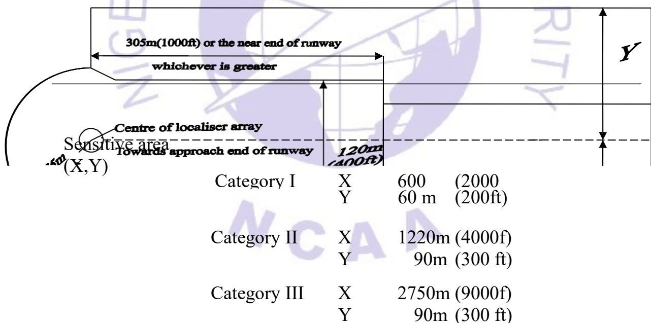
FIG. 2.1 Typical localiser critical and sensitive areas
